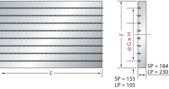
T-slot Dimensions
