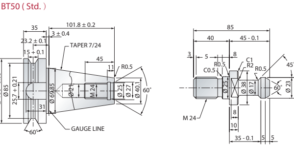
Tool Shank and Pull Stud Dimensions
