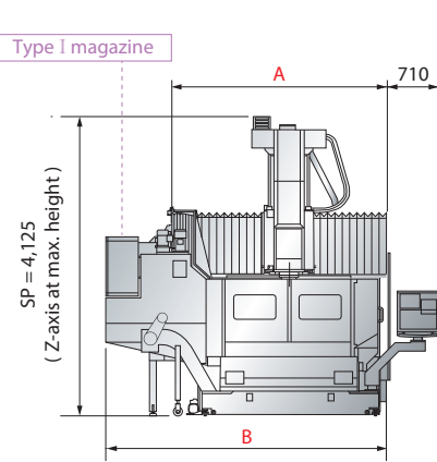
Machine Dimensions
